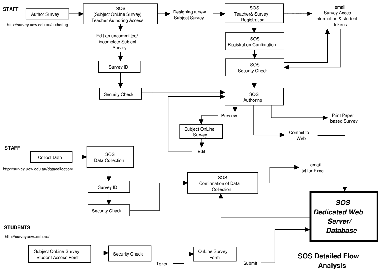
Fig 2 SOS Structure
